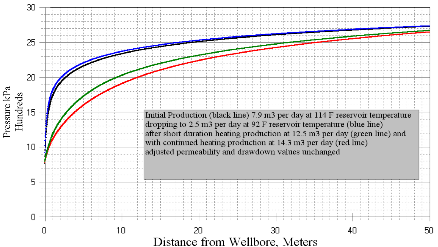
Bahrain 480 Pressure Profile
